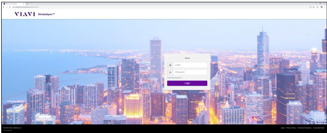
Figure 1: Stratasync Login
